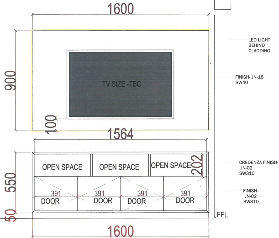
FRONT VIEW- CREDENZA WITH TV CLADDING-01
